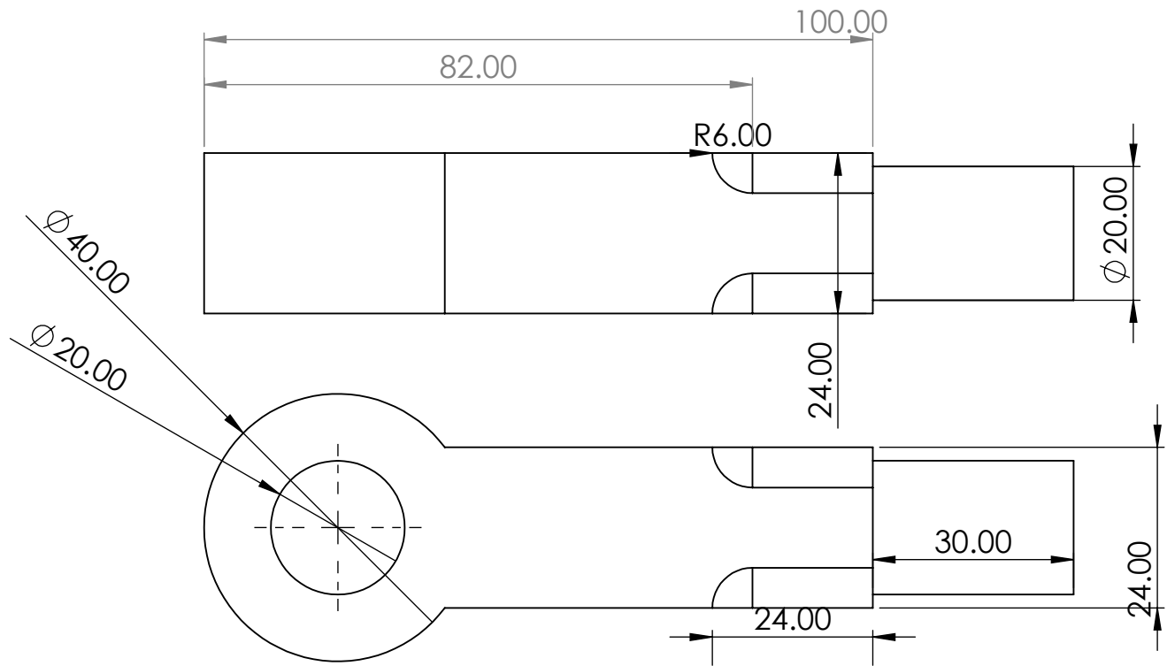
Eye End
