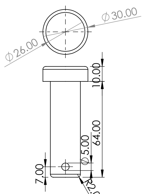
Knuckle Pin
