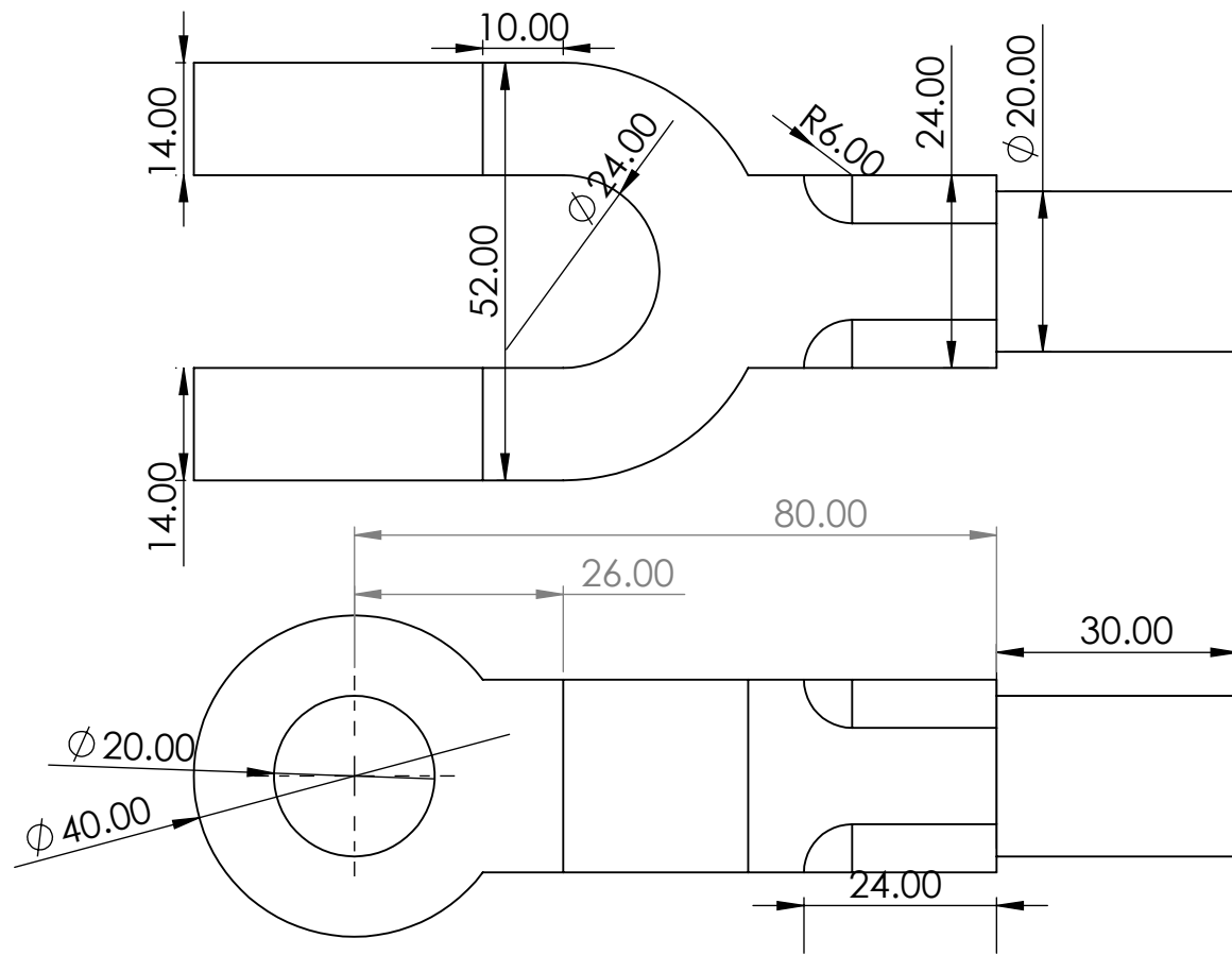
Fork End
